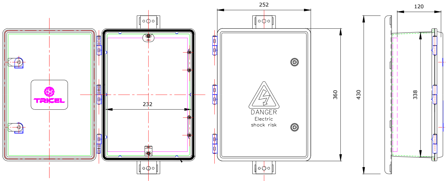
VIEW OF OPEN ASSEMBLED BOX AND DOOR
