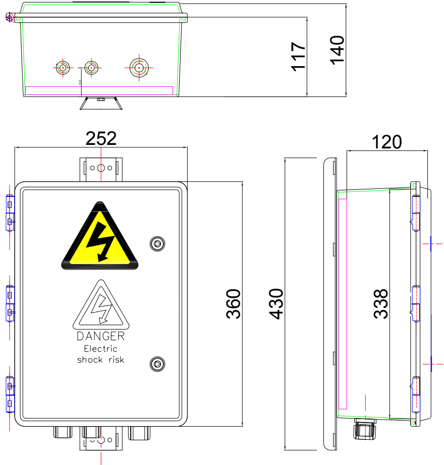
Detailed Sales Drawing
