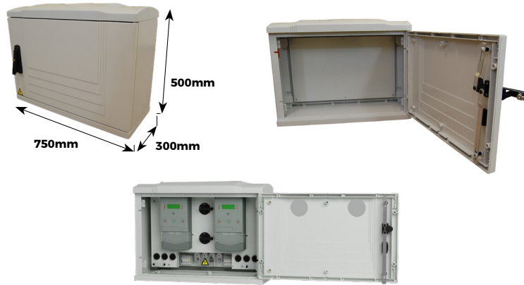
Example: 2 triphase metering box
