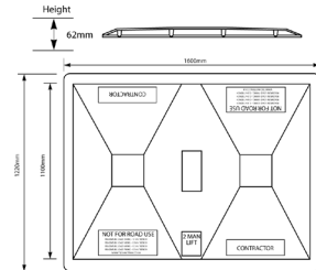
TRENCH COVER 1600X1220MM 1703001
