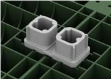
Multiple-layer connector for installation in multiple-layer systems between different layers, for connecting layers with each other
