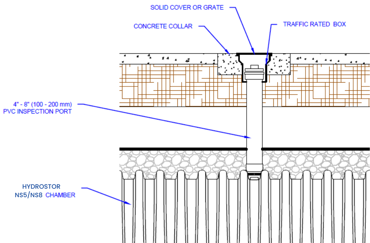
Figure 18 - Inspection Ports
