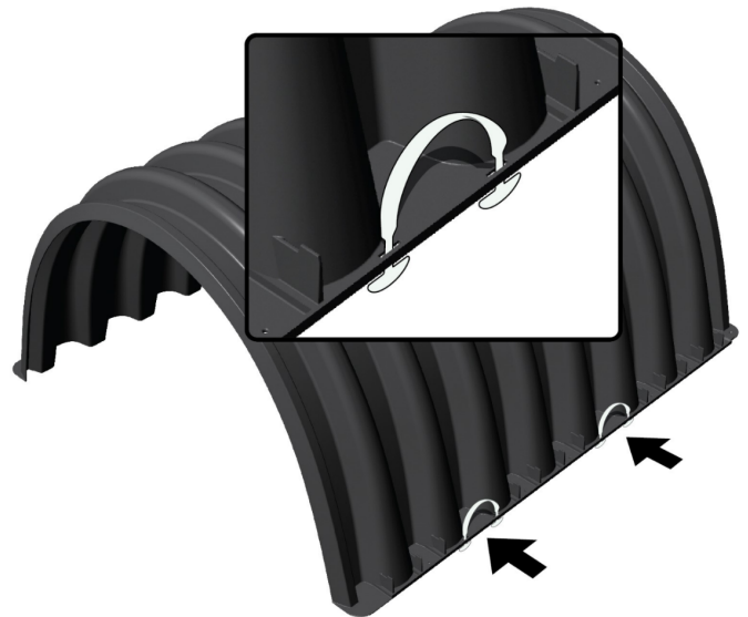
Figure 3 - Chamber Handles
